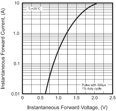
Fig.3 - Typical Instaneous Forward Characteristic
